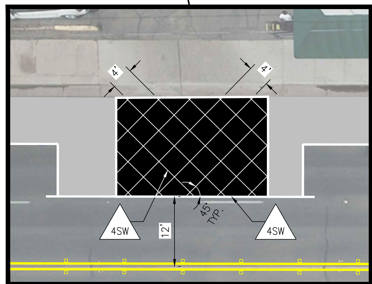
TYPICAL DRIVEWAY CROSSHATCH DETAIL NTS
