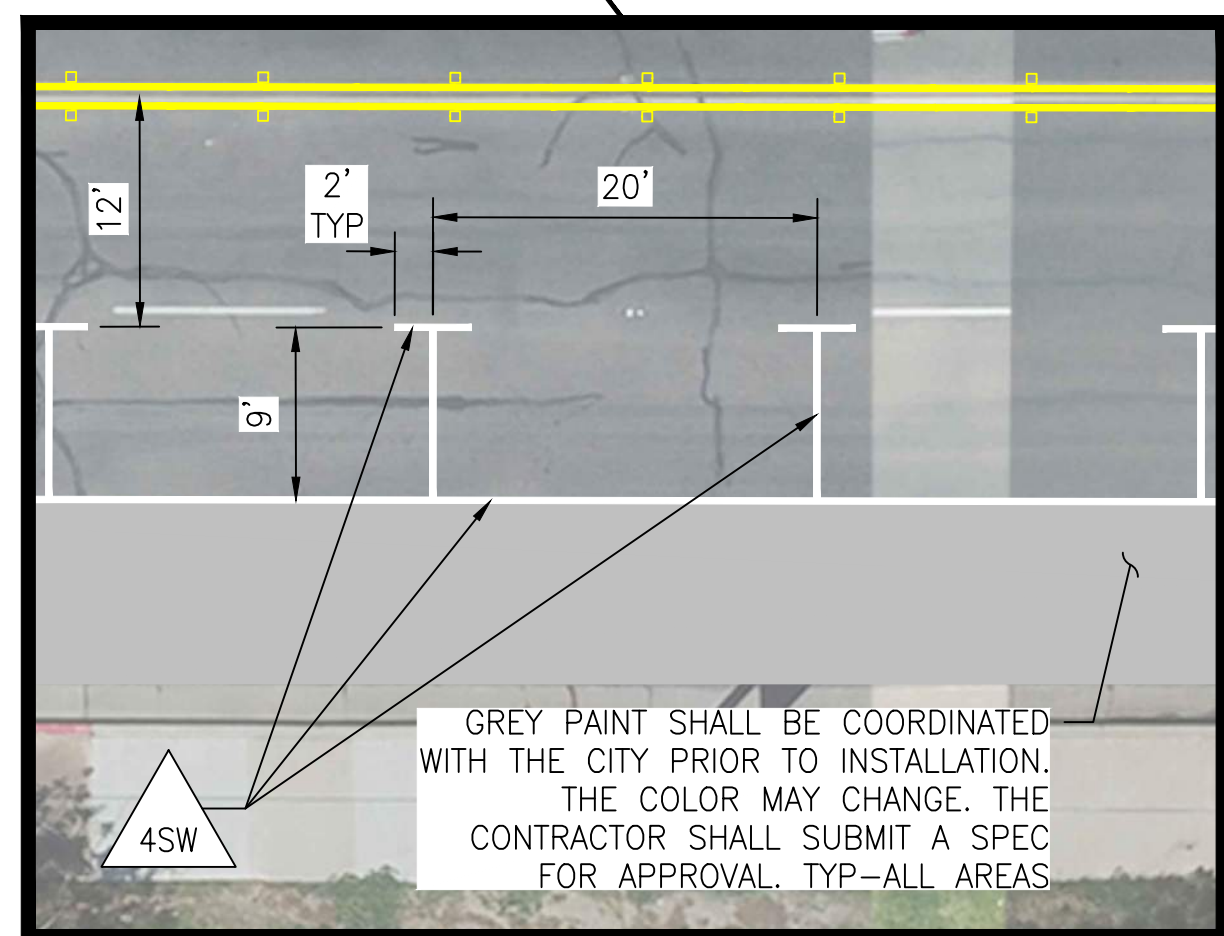
TYPICAL STANDARD PARKING DETAIL NTS
